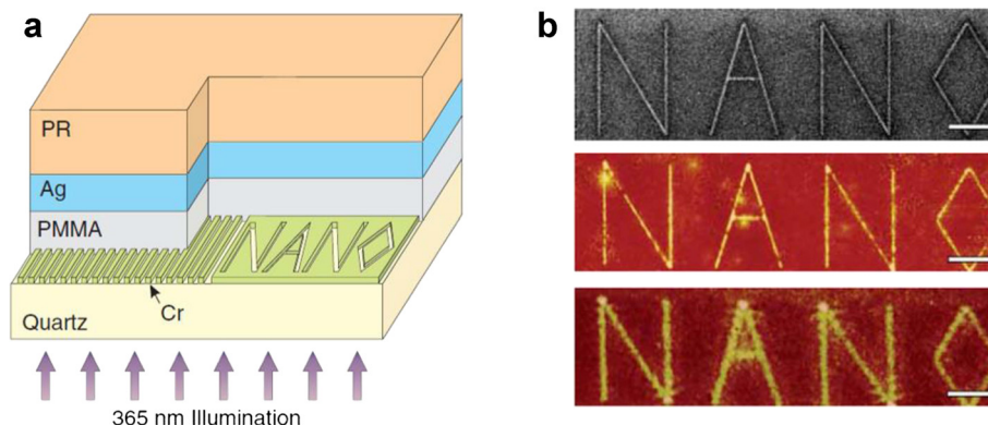
Fig. 5 The first experimental demonstration of near-field superlens. a Experimental set-up. 60 nm-wide slots of 120 nm pitch and letters ‘NANO’ whose linewidth is 40 nm are inscribed onto chrome. Here, silver slab functions as a superlens. b Experimental results. Top: FIB image of the object. Middle: AFM image of the image with the superlens. Bottom: AFM image of the image when the superlens was replaced by PMMA spacer. (The scale bars indicate 2 \mu\text{m} ) [52]
